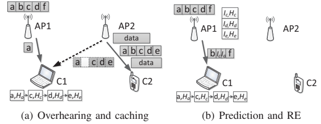
Fig. 2. PRECO in multiple AP infrastructure.
